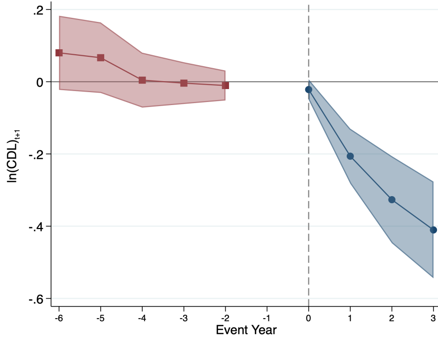
Figure A.6: Alternative Estimator. This figure plots the estimated coefficients and the associated 95% confidence intervals for dynamic treatment effects using the Sun and Abraham (2021) estimator. The treated units consist of zip codes which had AV testing during the sample period. The control units are the never-treated zip codes. The outcome variable is the natural log of the number of Class A commercial driver licenses in a zip code. The specifications include fixed effects for each zip code and fixed effects for the following groups, interacted with dummies for each year: county, median age, female share, non-white share, bachelor's degree share, population density, median earnings, and network-weighted density and earnings. Standard errors are clustered at the zip code level.
