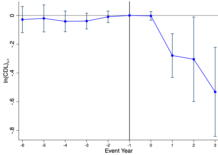
Figure A.5: Log Difference-in-Differences. This figure plots coefficients estimated from a stacked difference-in-differences analysis based on whether AV testing took place within a zip code (treated) as of the sample period. The control units are the never-treated zip codes. The outcome variable is the natural log of the number of Class A commercial driver licenses in a zip code. The specifications include zip code by stack and year by stack fixed effects and fixed effects for the following groups, interacted with dummies for each year: county, median age, female share, non-white share, bachelor's degree share, population density, median earnings, and network-weighted density and earnings. Standard errors are clustered at the zip code level.
